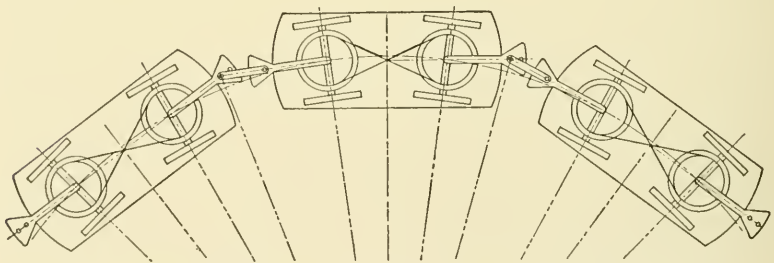
Fig. 6. Diagram Showing Steering Control of Schiemann Trackless Trolley Train
